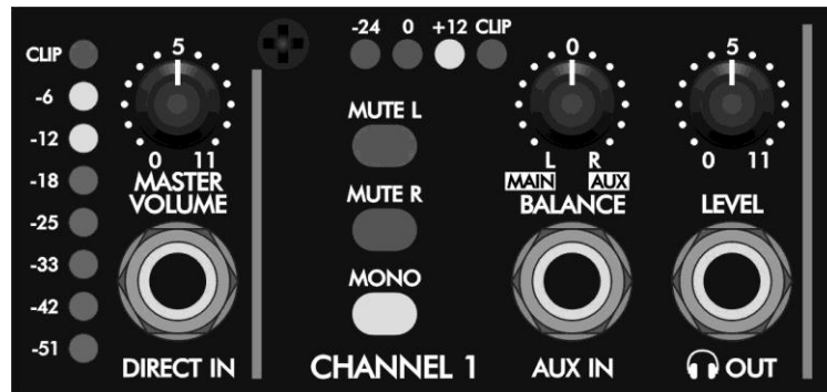
FIGURE 1 - Master Volume, Direct In, and Channel One
